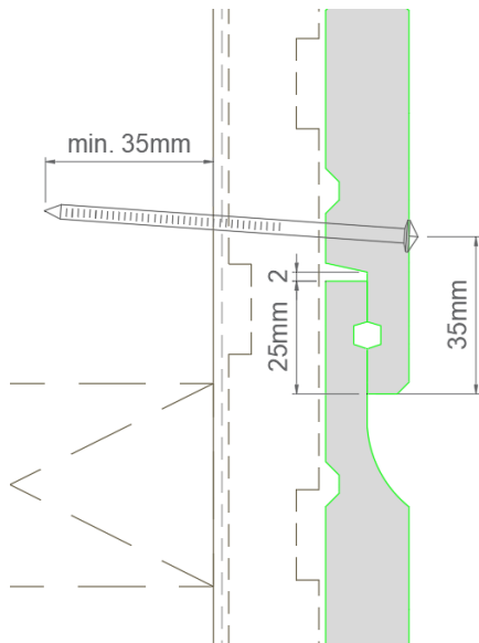
Figure 1 - Typical Rusticated Weatherboard Installation
