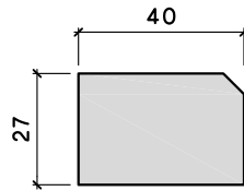
J32 Eaves Mould
