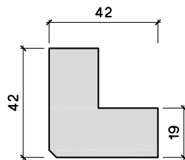
J42 External Corner Mould
