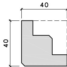
J40 External Corner Mould
