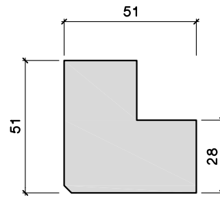
J45 External Corner Mould
