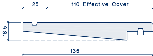
J65 Splaycut Weatherboards - 110mm Cover
